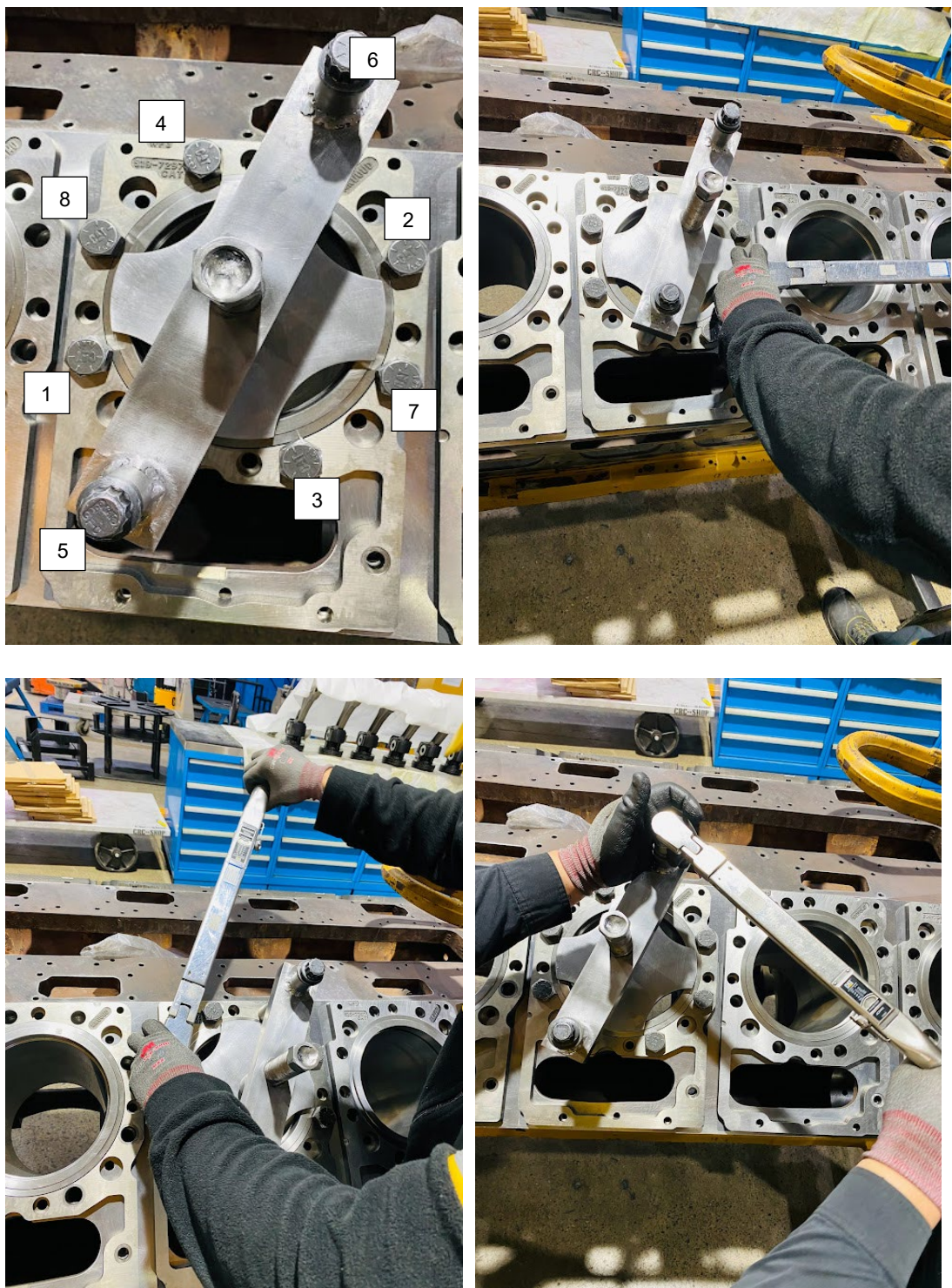
Illustration #11,12,13 and 14 bolt tightening torque is 95 Nm (70lb ft) in the numbered order in illustration #11.
